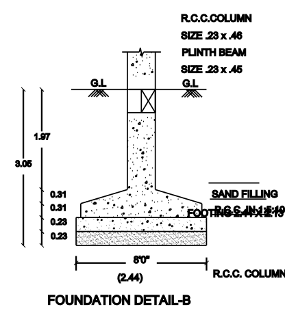
FOUNDATION DETAIL-B
