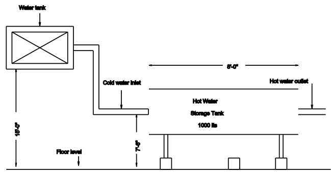
SOLAR WATER HEATER DETAIL
