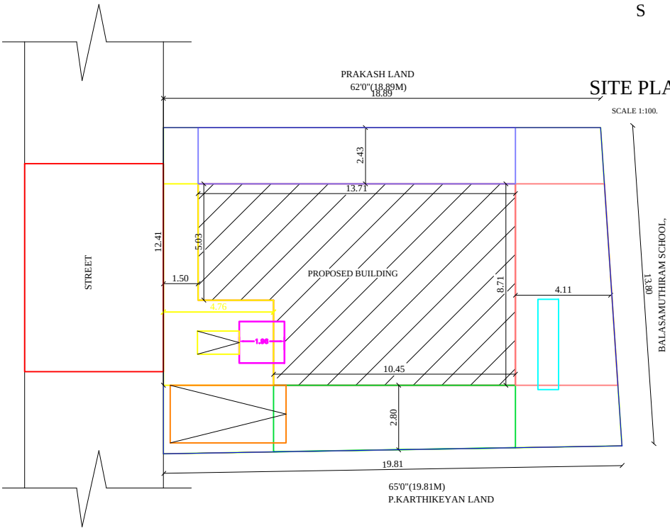
SET BACK DETAILS
