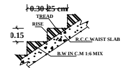
CTION OF STAIRCASE
