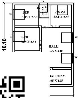
PROPOSED FLOOR PLAN
