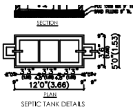
SEPTIC TANK DETAILS
