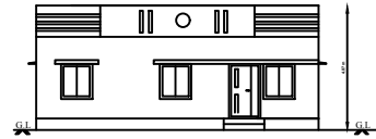
FRONT ELEVATION
