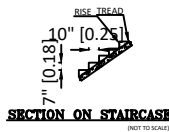
SECTION ON STAIRCASE (NOT TO SCALE)
