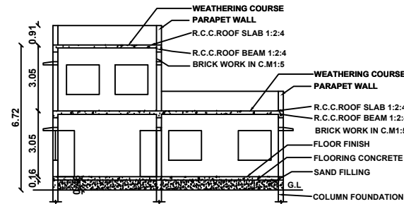
SECTION ON GG
