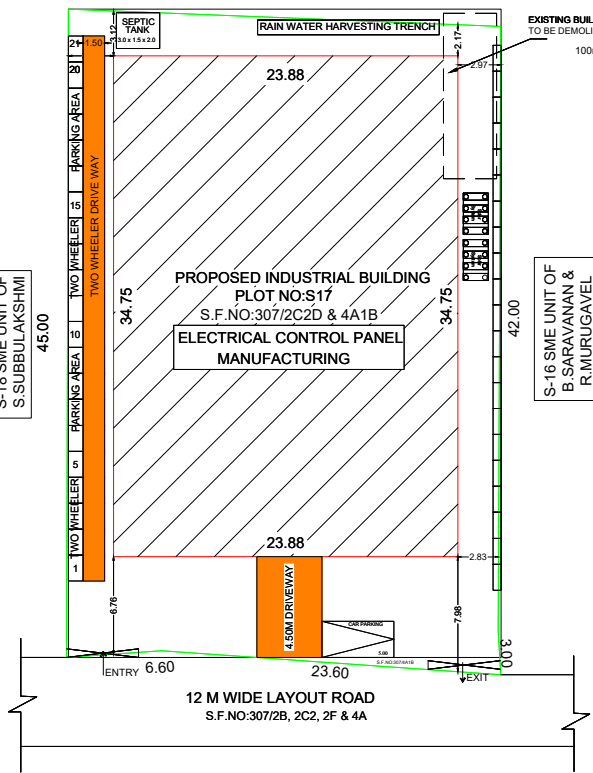
RAINWATER HARVESTING RWH_CAPACITY_L=3000LTRS
