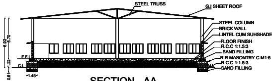
SECTION - AA FOR INDUSTRIAL BUILDING
