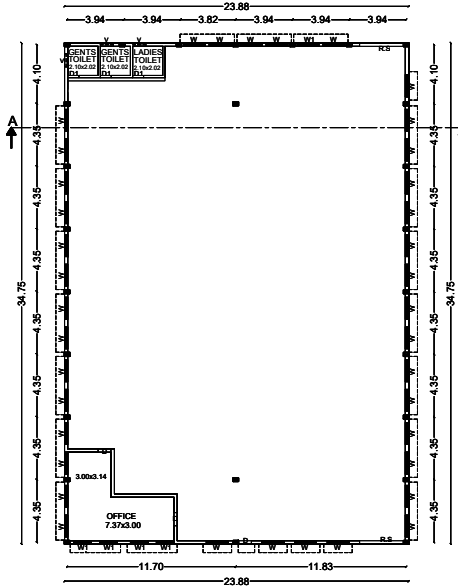
PLAN FOR INDUSTRIAL BUILDING
