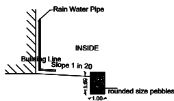
RAINWATER HARVESTING RWH_CAPACITY_L=3000LTRS
