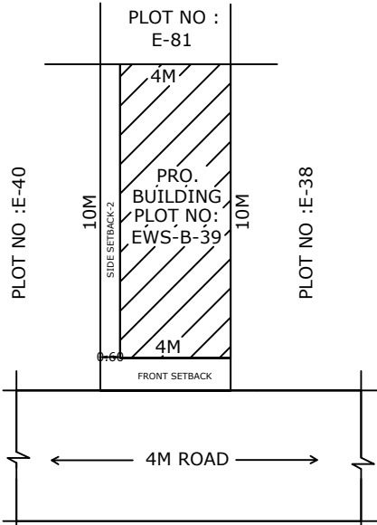
SITE PLAN
