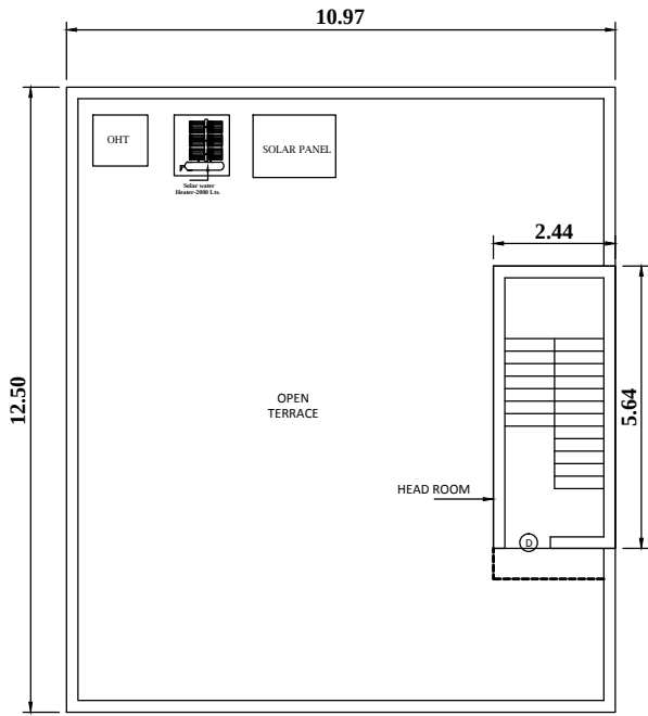
GROUND FLOOR ROOF PLAN
