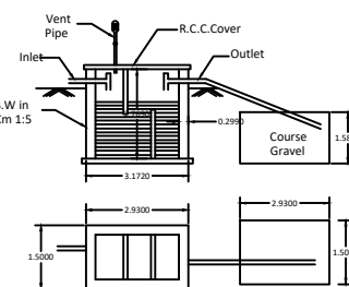
SEPTIC TANK & D-TRENCH DETAILS
