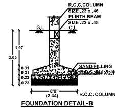
FOUNDATION DETAIL-B
