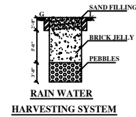
RAIN WATER HARVESTING SYSTEM
