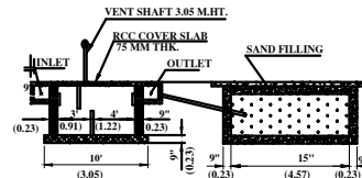
SECTION ON SEPTIC TANK & DISP-TRENCH
