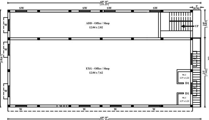
ADD & EXG - FIRST FLOOR PLAN
