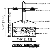
COLUMN FOUNDATION
