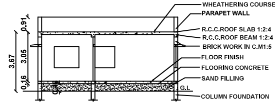
SECTION ON GG
