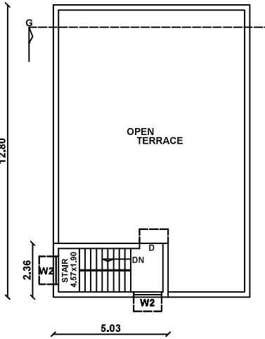
HEAD ROOM PLAN
