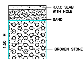
N WATER HARVEST COLLECTION PIT.
