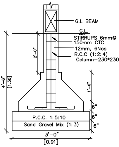
R.C.C. COLUMN FOOTING DETAILS SCALE : 1:25
