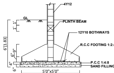
R.C.C.COLUMN FOOTING DETAIL
