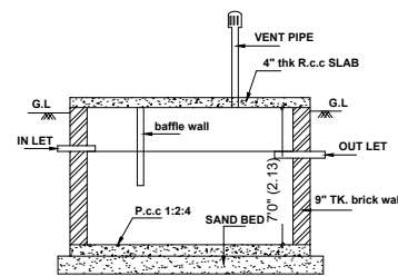
SECTION AT P-Q
