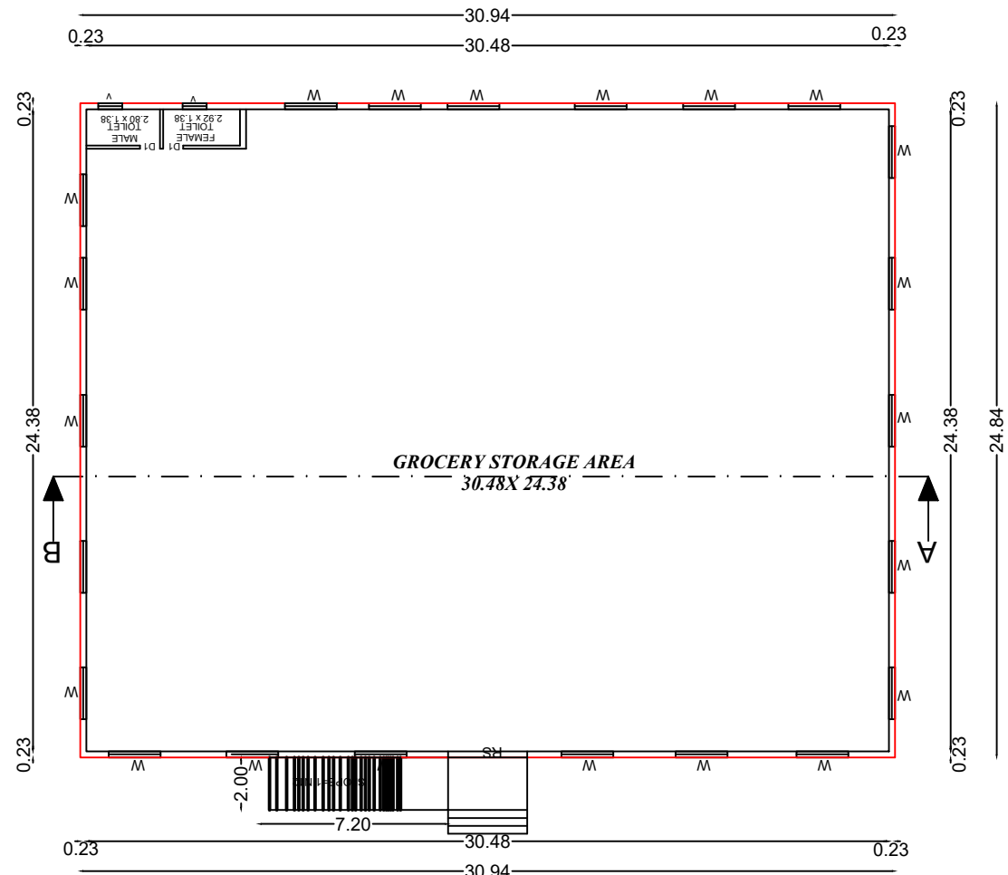
GROUND FLOOR BLOCK -1
