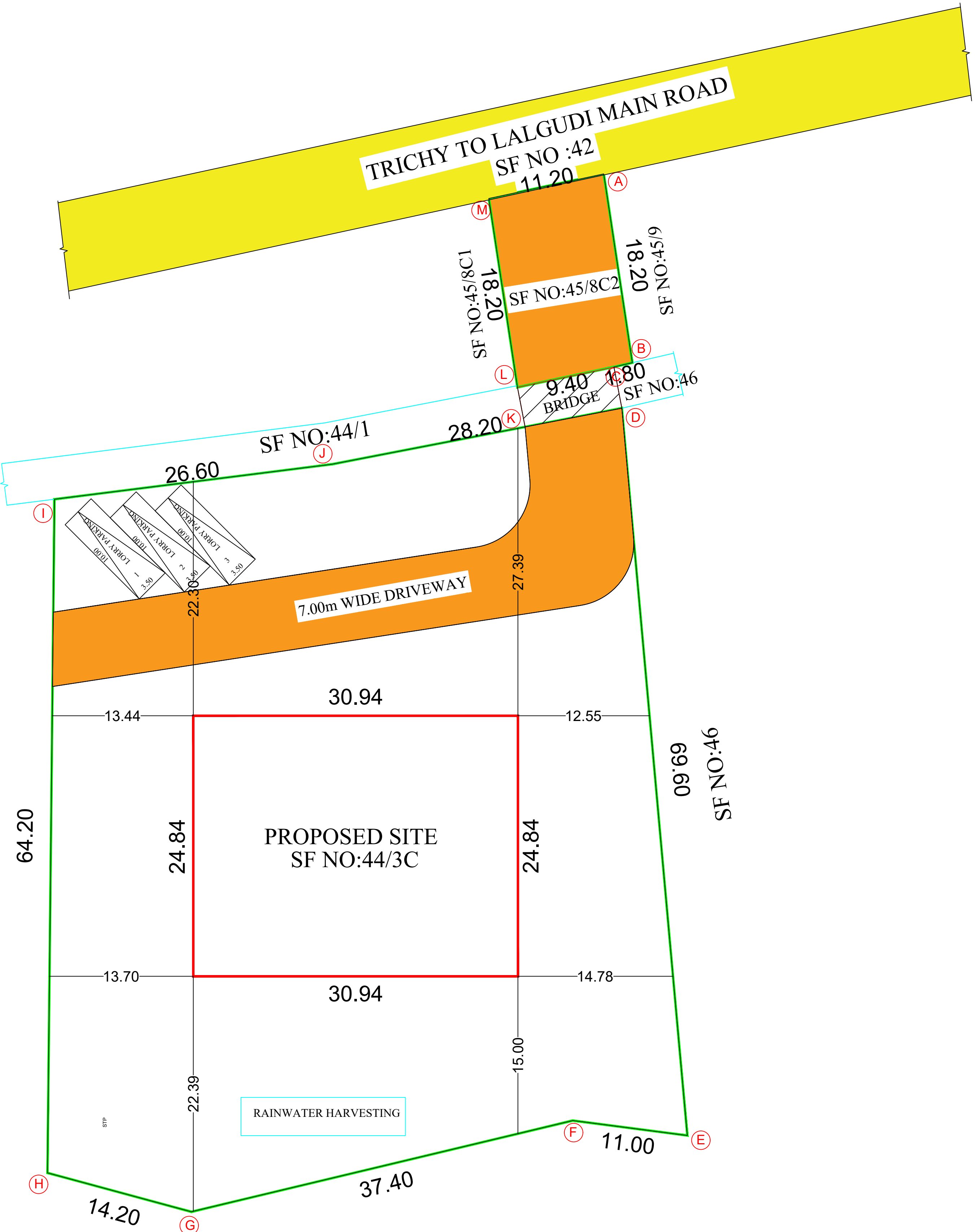
SITE PLAN
