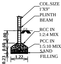
COLUMN DETAILS
