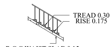
R.C.C WAIST SLAB 0.15 STAIRCASE DETAILS
