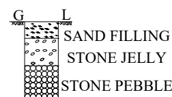
RAINWATER HARVESTING PIT
