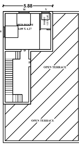
PRO. SECOND FLOOR PLAN
