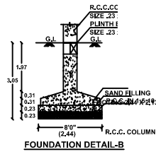
FOUNDATION DETAIL-B
