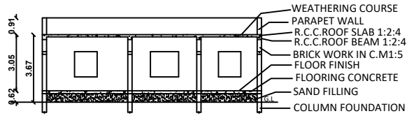
SECTION- SS
