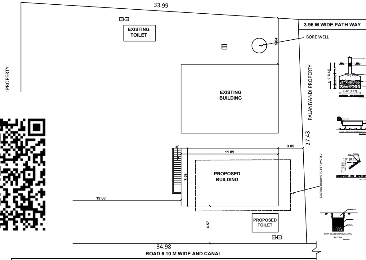
SITE PLAN
