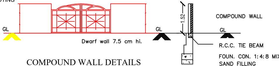
SECTION
