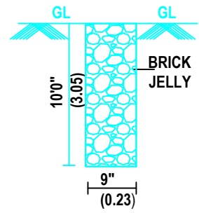
PERCOLATION PIT
