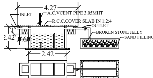
SECTION SEPTIC TANK & DISPERSION TRENCH
