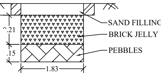
N WATER HARVESTING PIT
