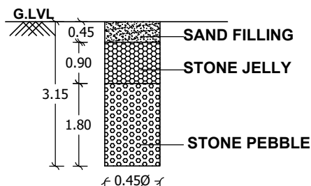
RAIN WATER HARVESTING PIT (NOT TO SCALE)
