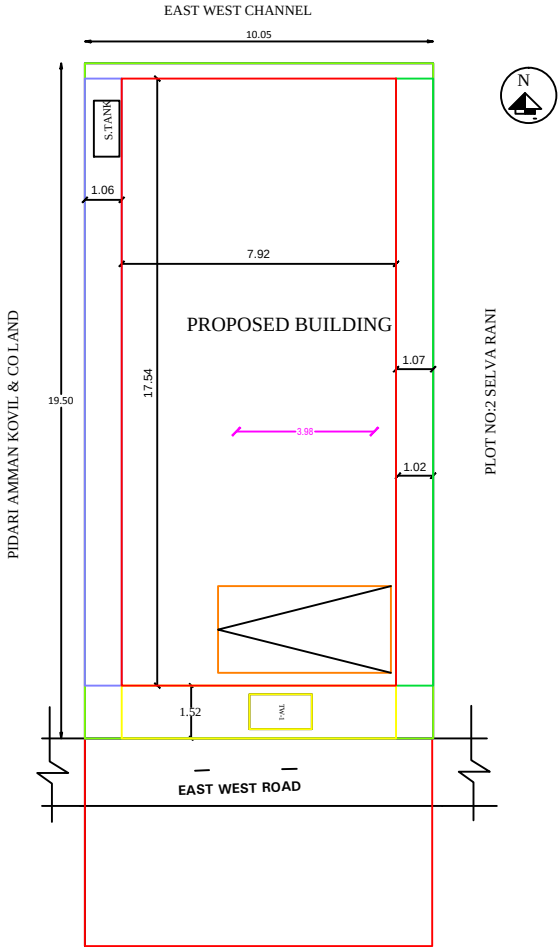
SITE PLAN
