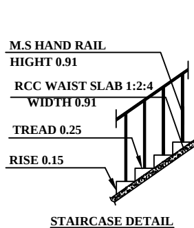
STAIRCASE DETAIL
