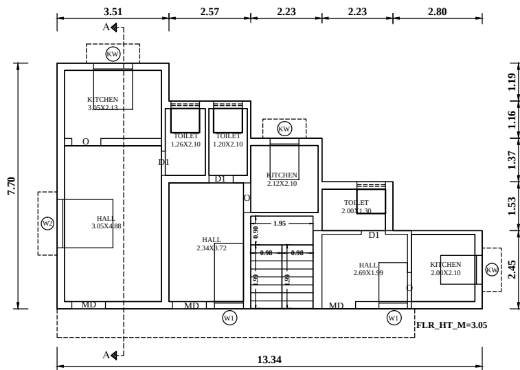
PRO FIRST FLOOR
