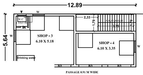
5T FLOOR PLAN
