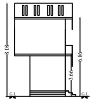
FRONT ELEVATION
