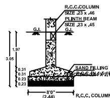
FOUNDATION DETAIL-E
