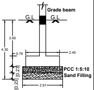
FOUNDATION DETAILS
