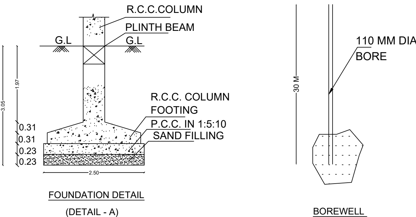
(DETAIL - A)
