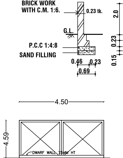
MAIN GATE ELEVATION
