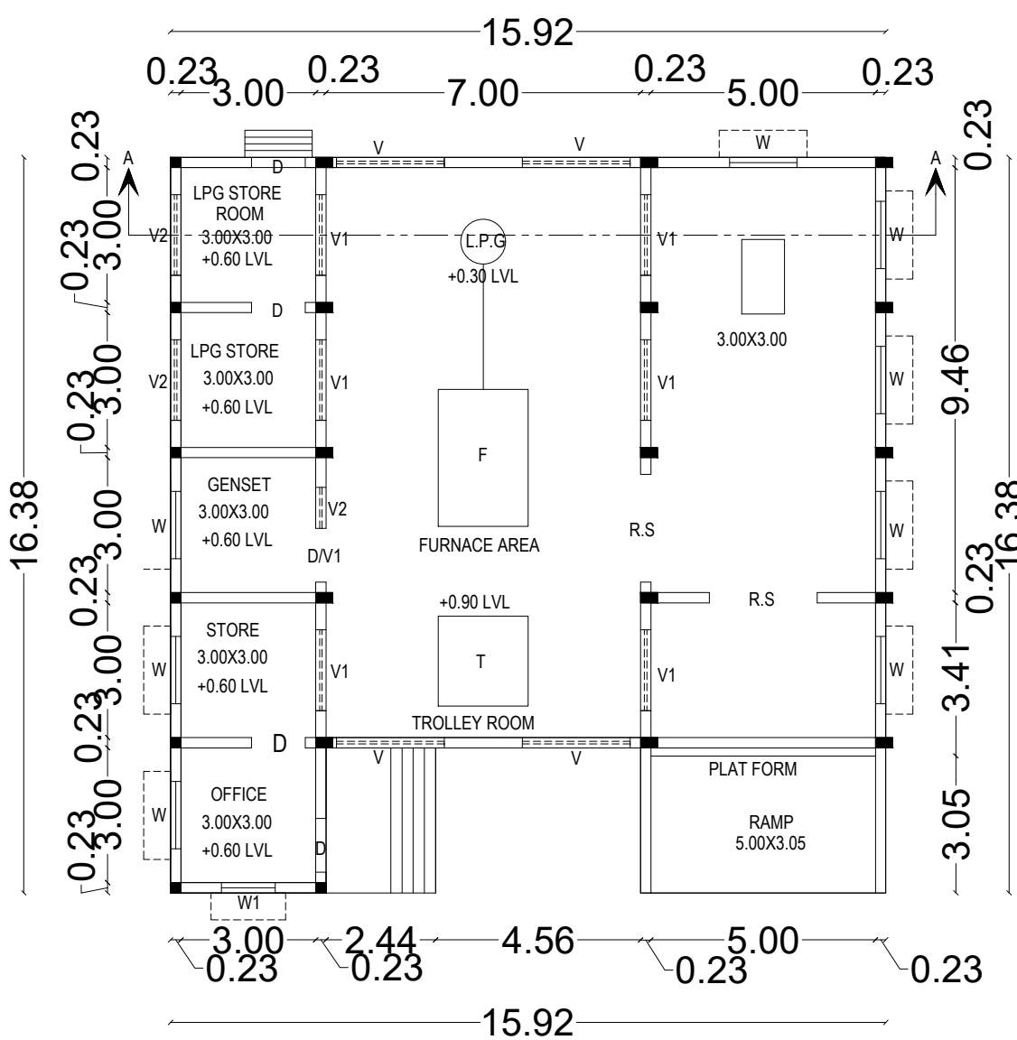
PLAN
