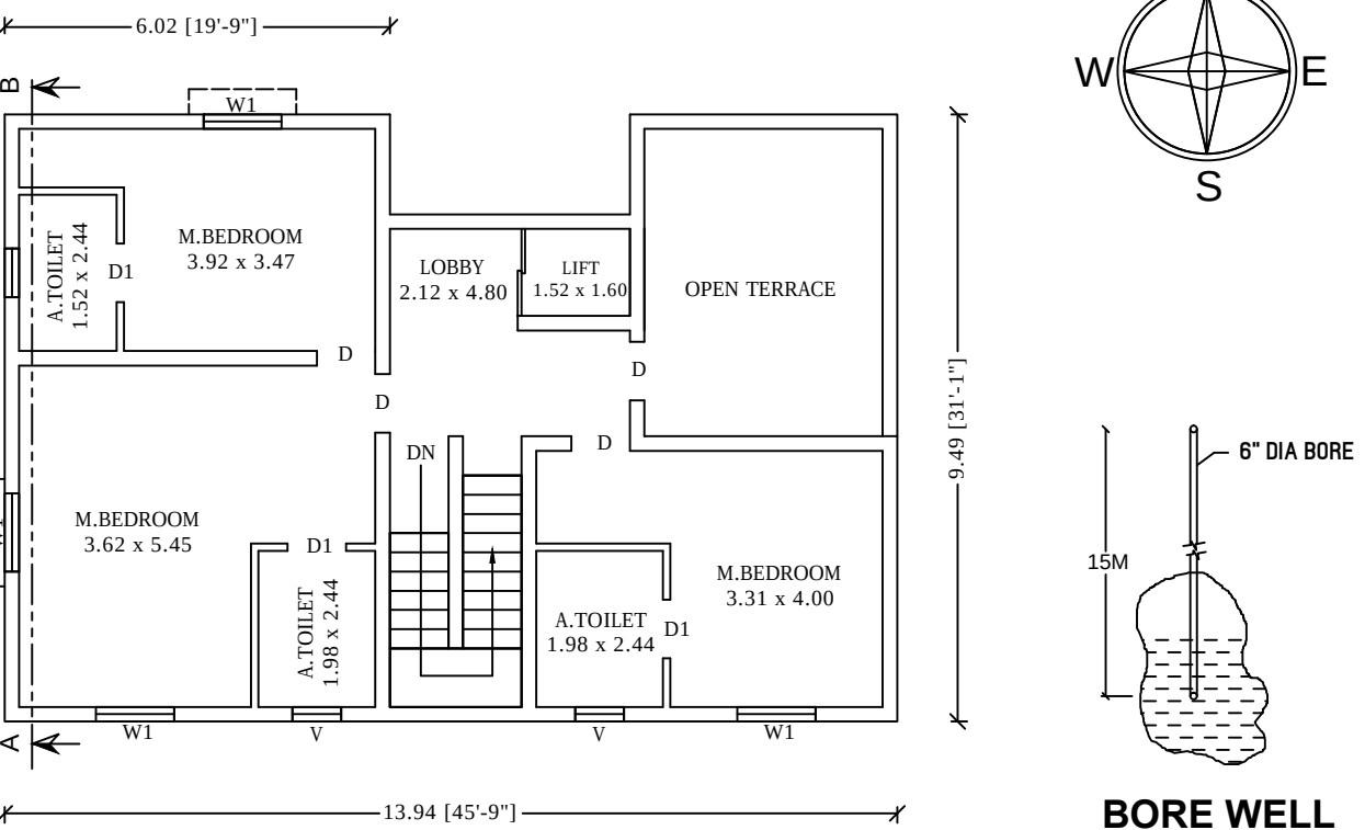
BORE WELL (NOT TO SCALE)
