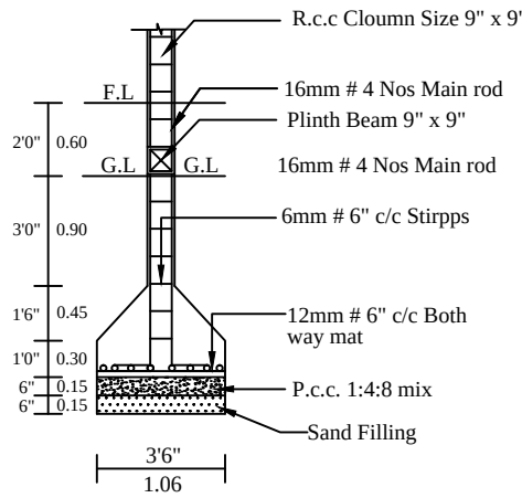
COLUMN DETAILS
