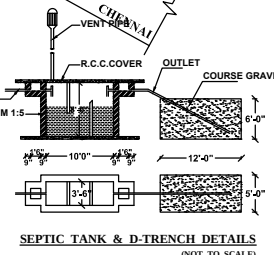
SEPTIC TANK & D-TRENCH DETAILS (NOT TO SCALE)
