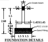
FOUNDATION DETAILS
