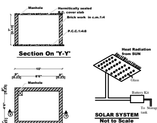
Sump Detail - Plan Scale -1:50
