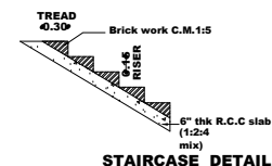
STAIRCASE DETAIL
