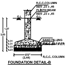
FOUNDATION DETAIL-B
