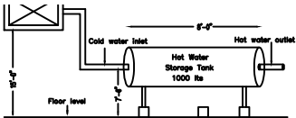
SOLAR WATER HEATER DETAILS
