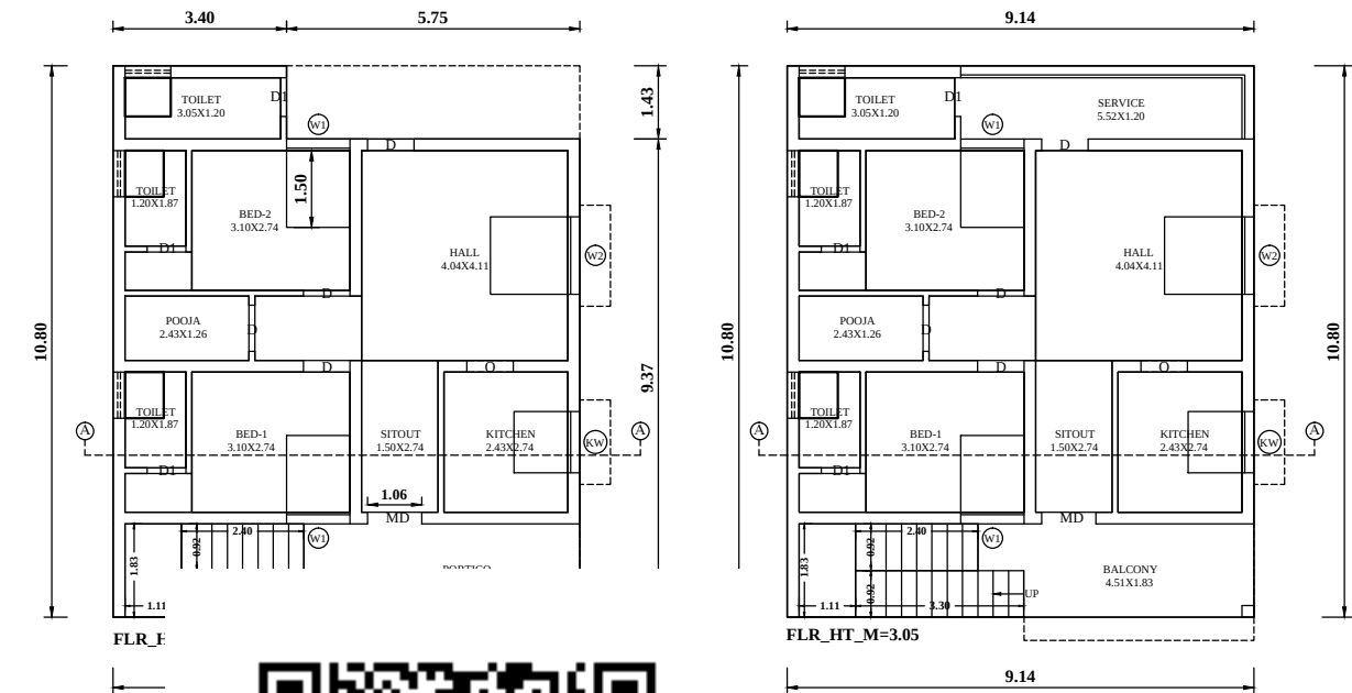
PRO FIRST FLOOR
