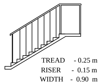
STAIRCASE DETAILS
