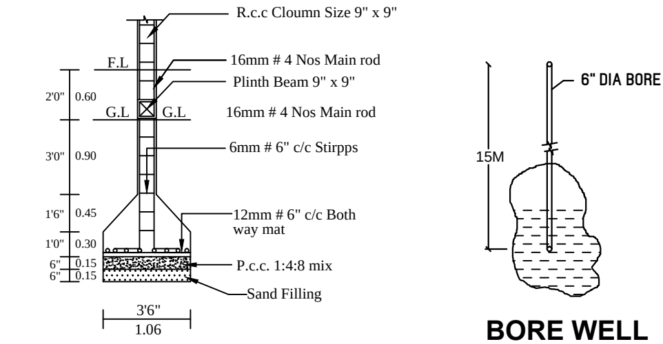
BORE WELL (NOT TO SCALE)
