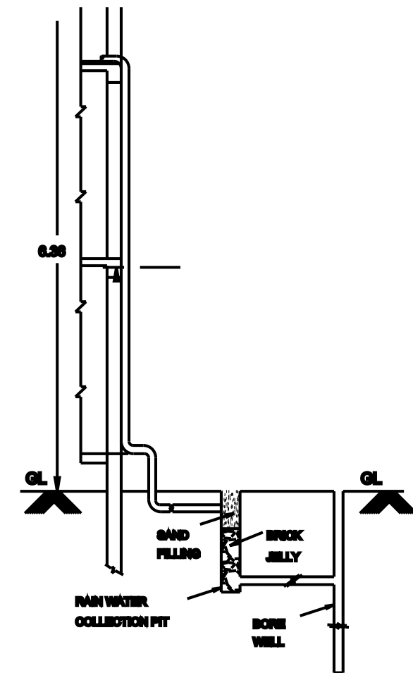
RAIN WATER HARVESTING SYSTEM RWH_CAPACITY_L=1000LTRS
