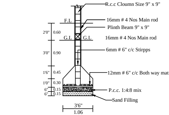
COLUMN DETAILS
