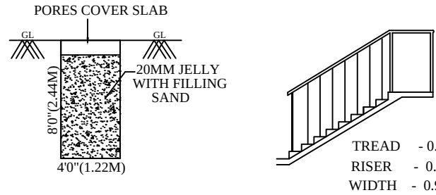
RAINWATER HARVESTING
