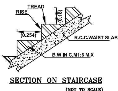
SECTION ON STAIRCASE
