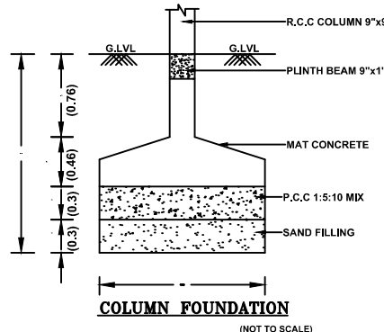
COLUMN FOUNDATION
