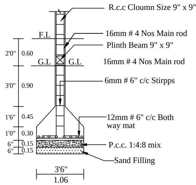
COLUMN DETIALS
