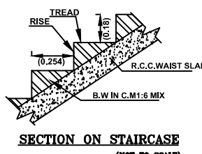
SECTION ON STAIRCASE
