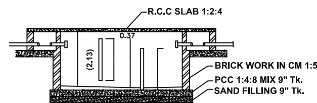
SECTION
