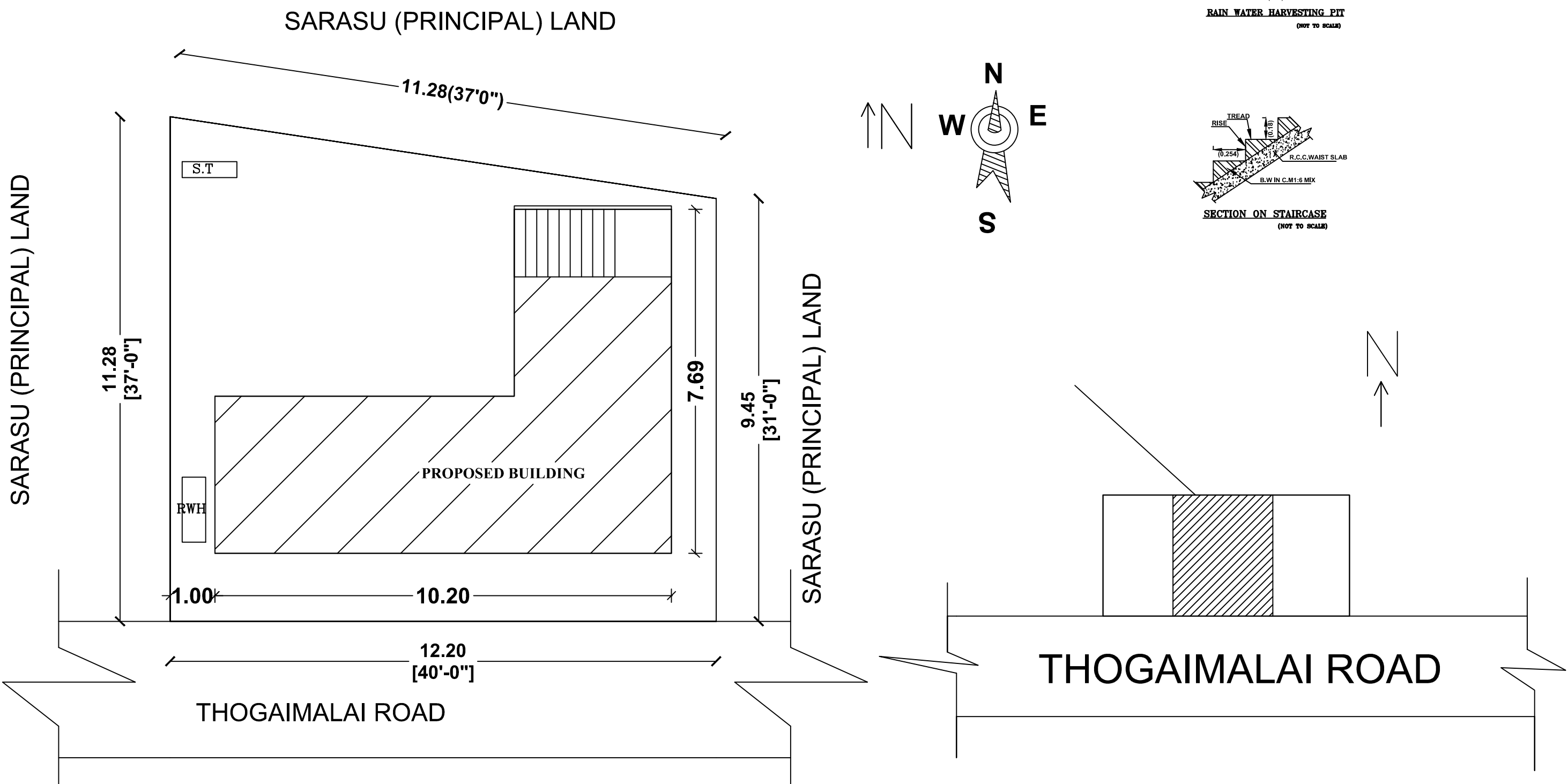
KEY PLAN
