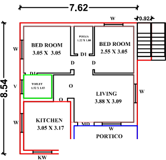
PRO. GROUND FLOOR
