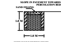
SLOPE IN PAVEMENT TOWARDS PERCOLATION BED
