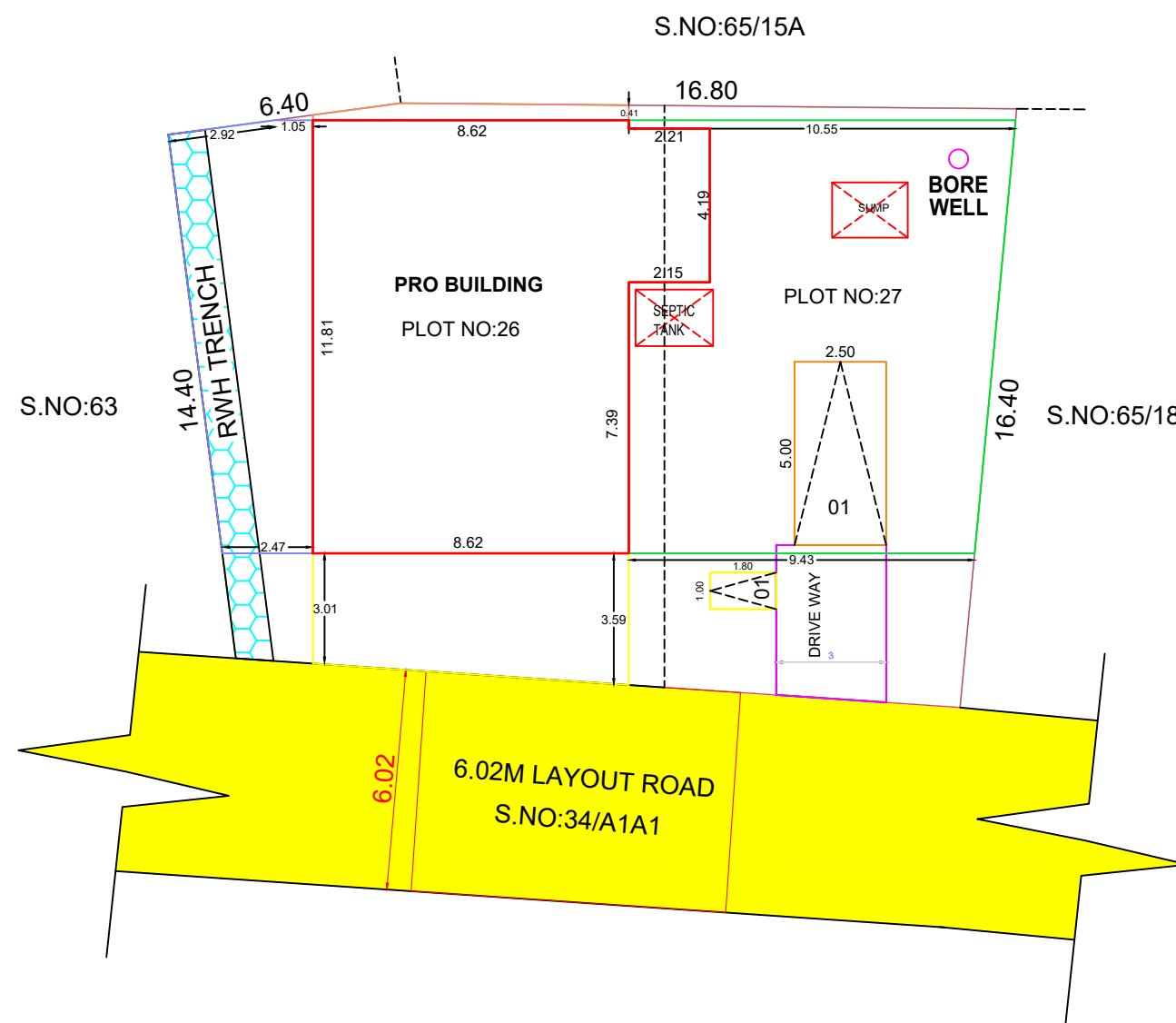
SITE PLAN
