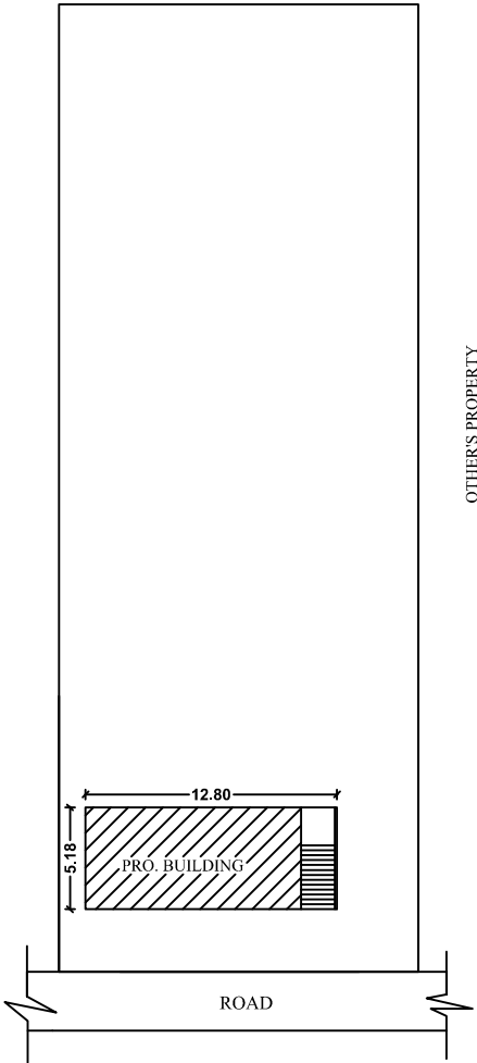
SITE PLAN
