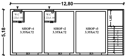
PRO.GROUND FLOOR PLAN
