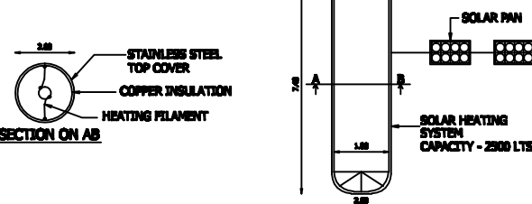
PLAN OF SOLAR WATER HEATING SYSTEM
