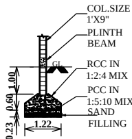
COLUMN DETAILS
