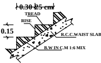
SECTION OF STAIRCASE
