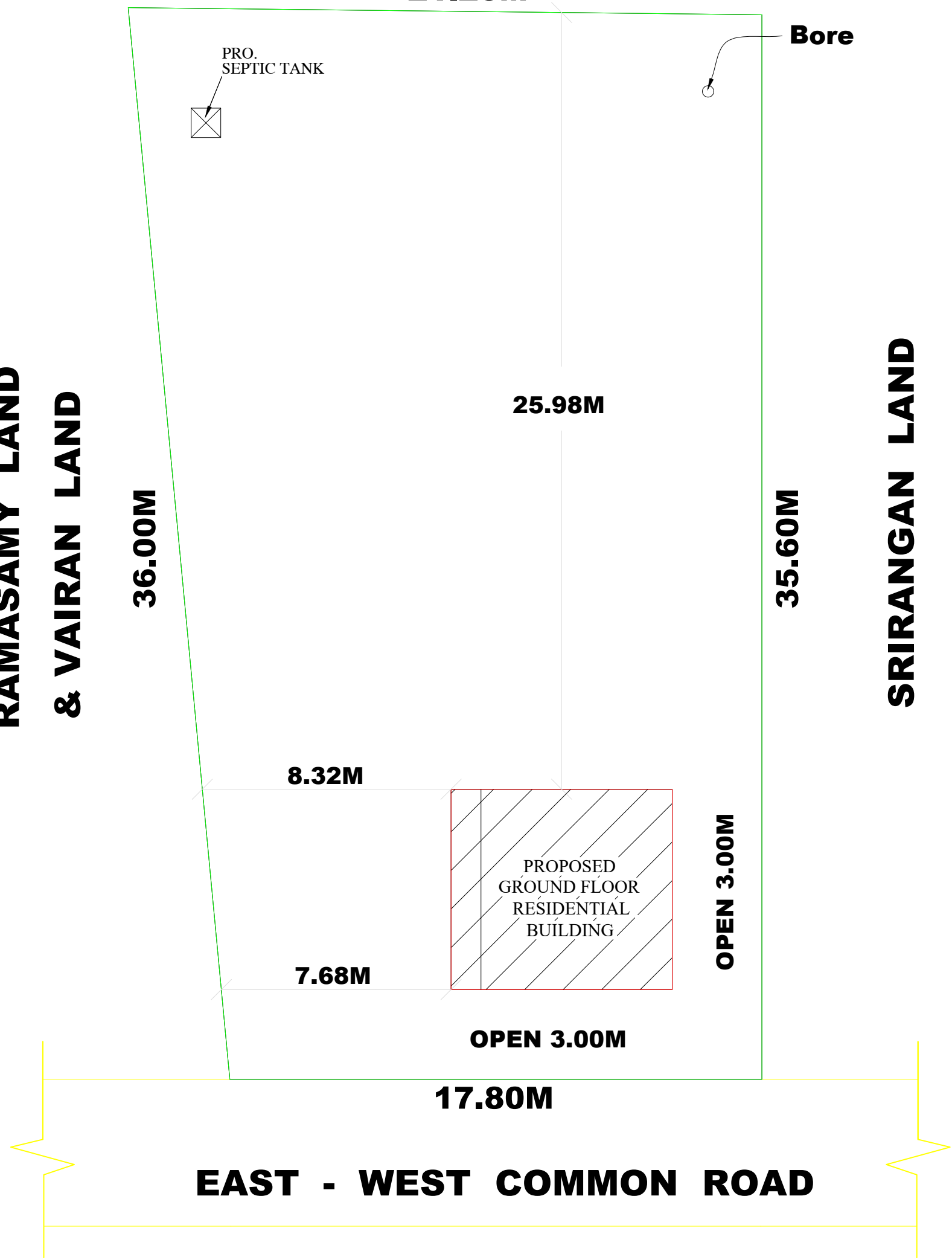
SITE PLAN (SCALE 1:1)
