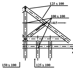
TRUSS DETAILS
