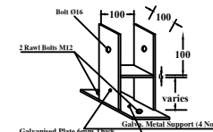
UPPER BOLTS DETAILS (IN MM)
